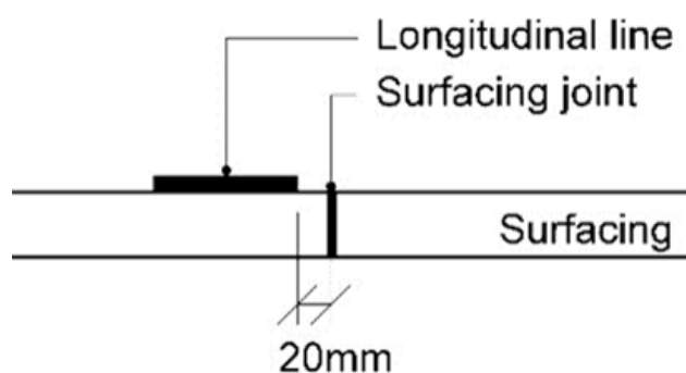
Figure 7.2(a): Longitudinal Line Offset from Surfacing Joint
