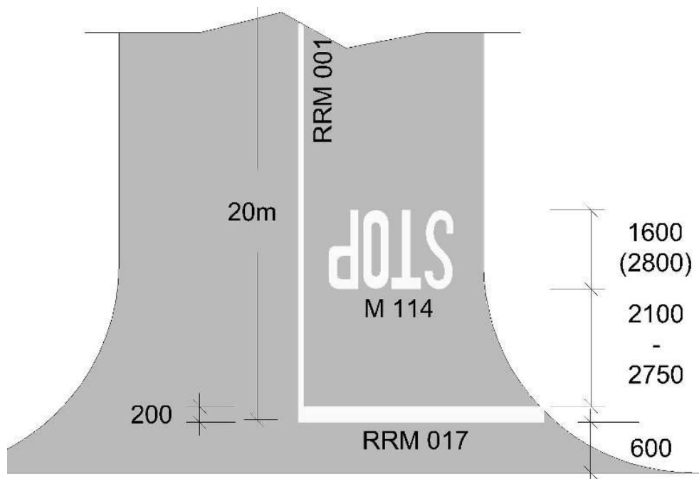
Figure 7.35: Example of Priority-Controlled Stop Junction
