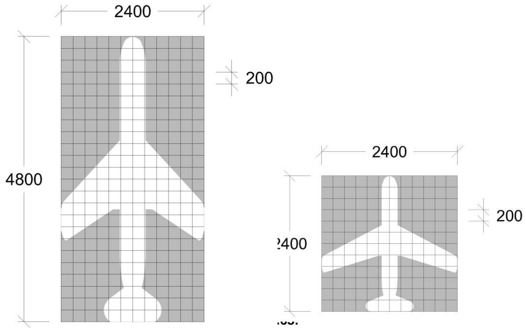
Construction of M 127 Airport Symbol
