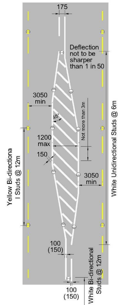
M104 Ghost Island at Crest
