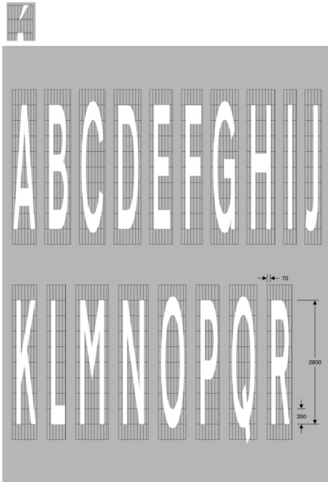
Figure 7.62: 2800mm Elongated Font
