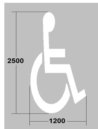
RRM 015: Disabled Persons' Parking Bay Symbol
