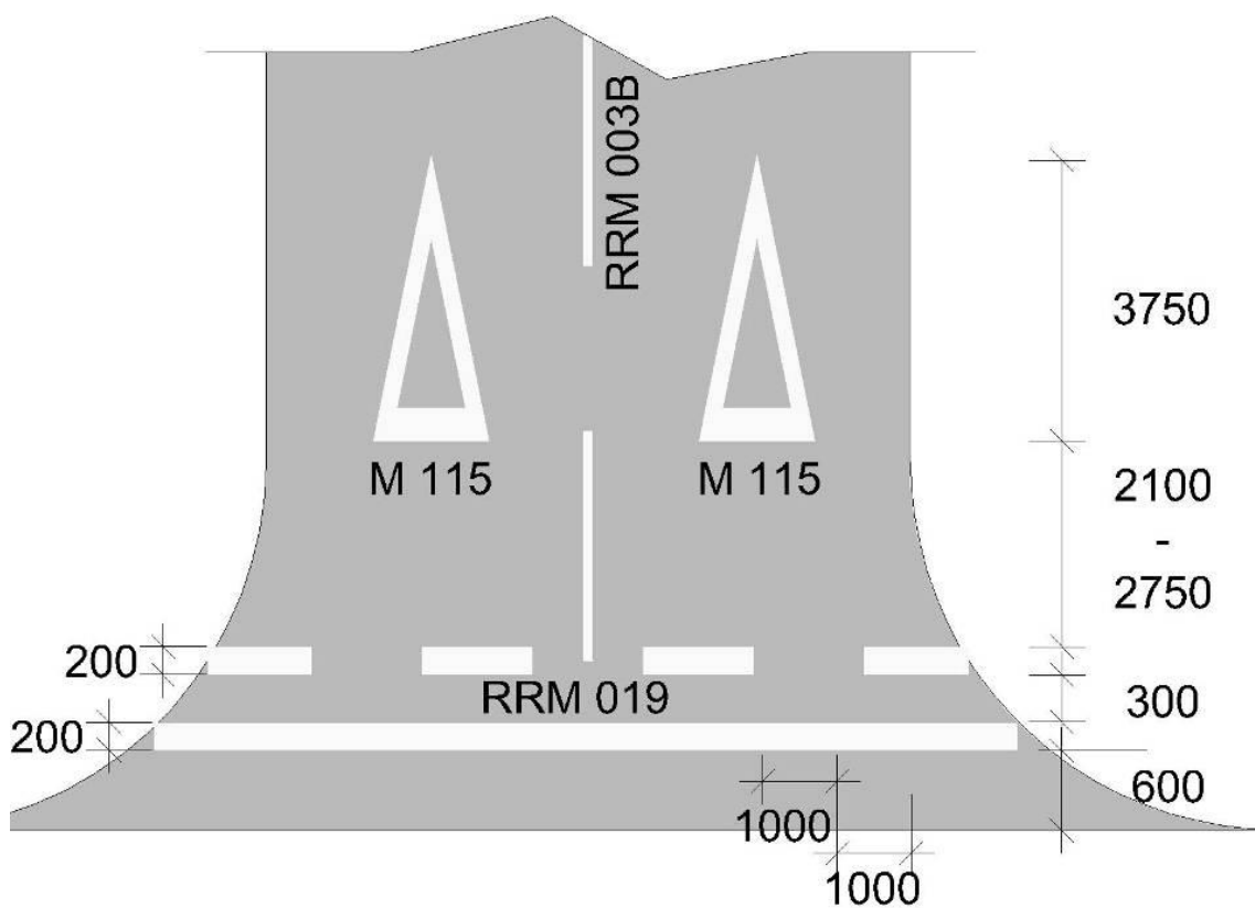
Figure 7.37: Example of Markings at Mouth of One-way Street
