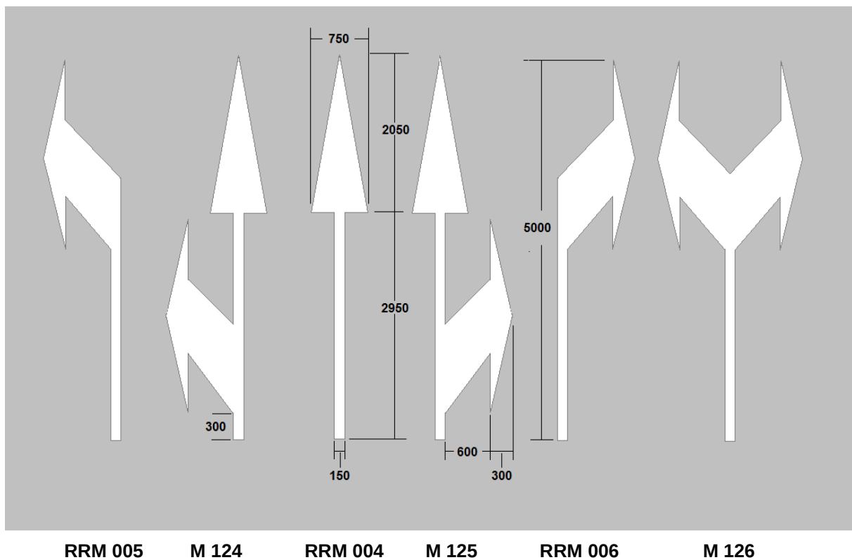
Figure 7.25: Lane Indication Arrows ( > 60\text{km/h} )
