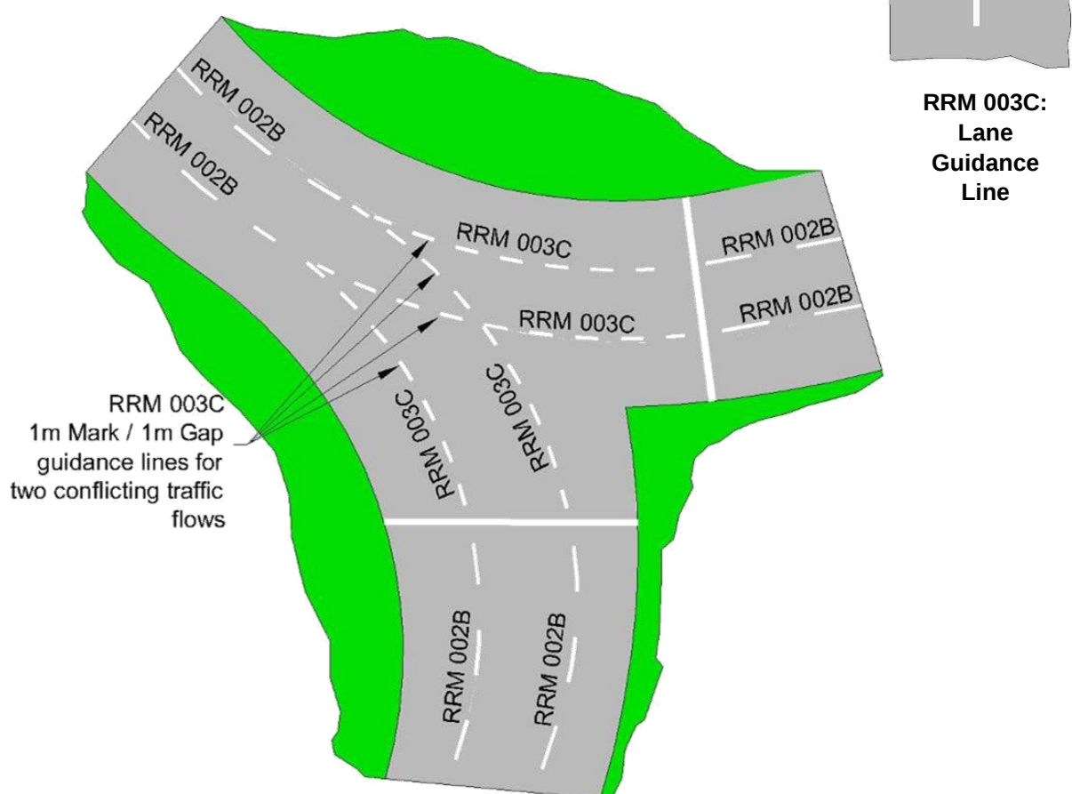
Figure 7.49: Use of Lane Guidance Line, RRM 003C, on a Signalised Roundabout
