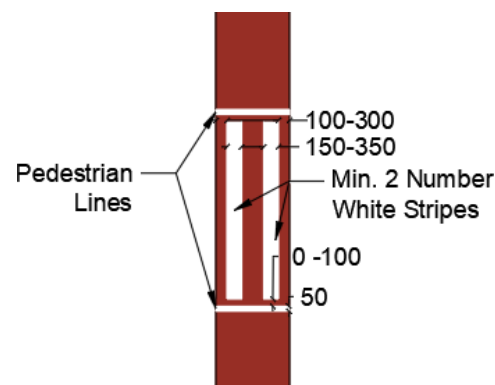
RPC 001B: Zebra Crossing of a Cycle Track
