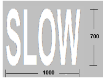
M106C Cycle Track SLOW Marking
