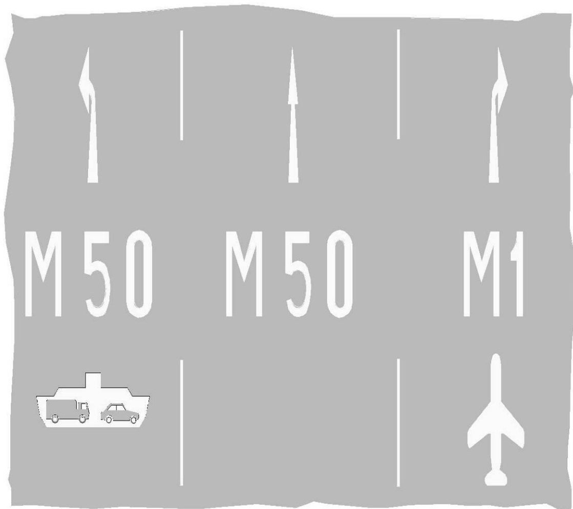
M 105: Typical Lane Destination Markings
