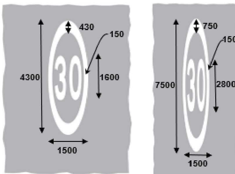
M 108: Speed Markings
