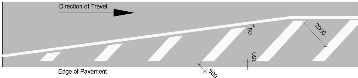
Diagonal Hatched Marking for Use on Offside of Motorways and Dual Carriageways
