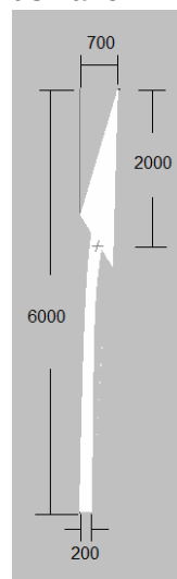
M 101: Right Deflection Arrow
