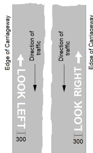
M 107: LOOK LEFT/RIGHT Marking
