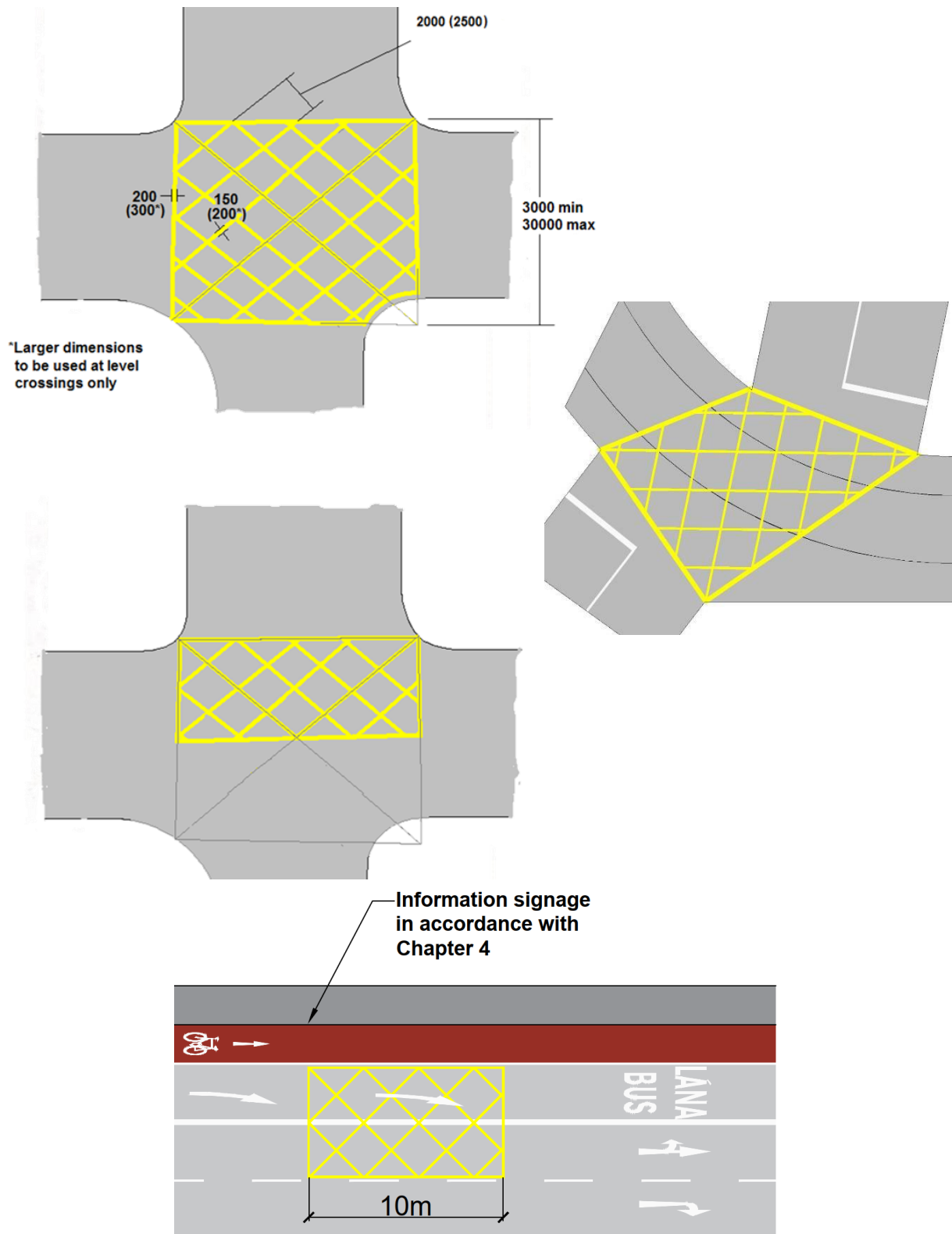
RRM 020: Yellow Box Markings
