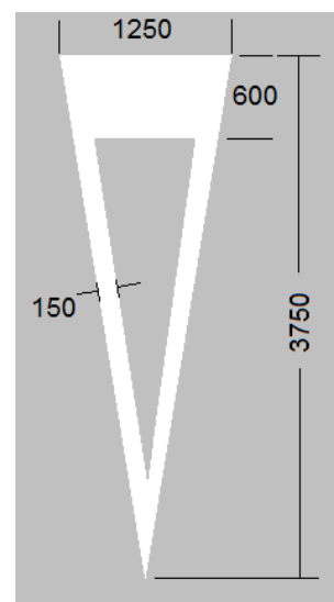
M 115: Triangular Yield Marking
