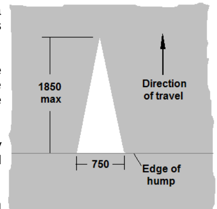
M 112 Traffic Calming Triangle
