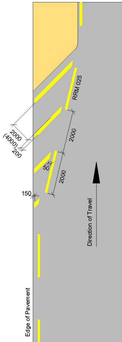
Figure 7.19: Hatched Marking on Nearside of Carriageway on Roads other than Motorways and Duals
