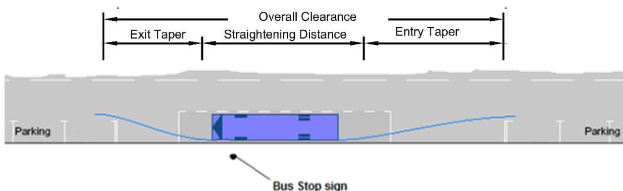
Figure 7.28: Clearance at Bus Stop Required for Parallel Docking
