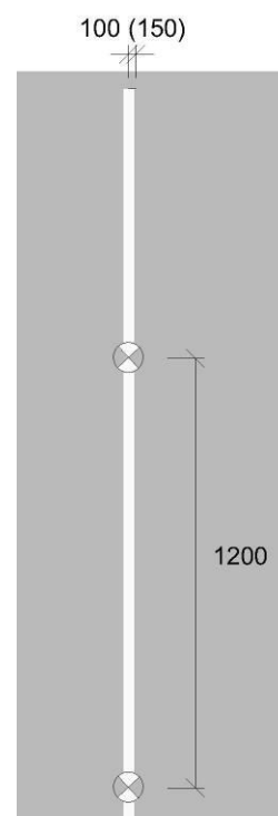
RRM 001: Continuous Single Centre Line
