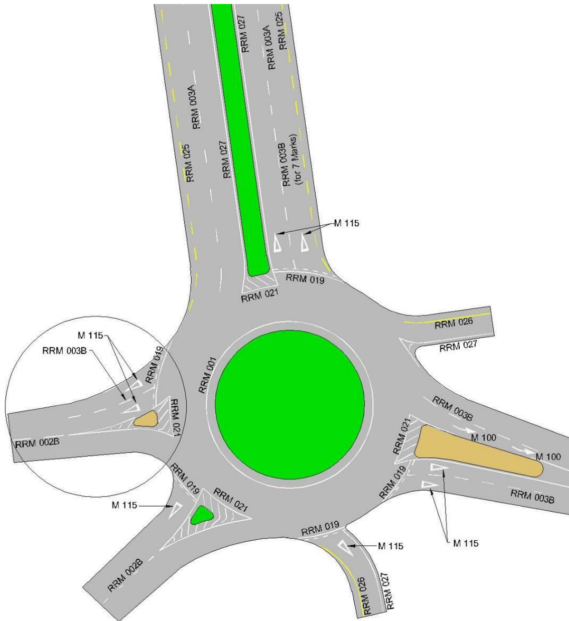
Figure 7.44: Markings at an Illustrative Roundabout
