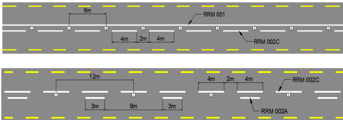
Figure 7.2(b): Double Line System
