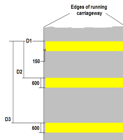
M 113: Yellow Bar Markings
