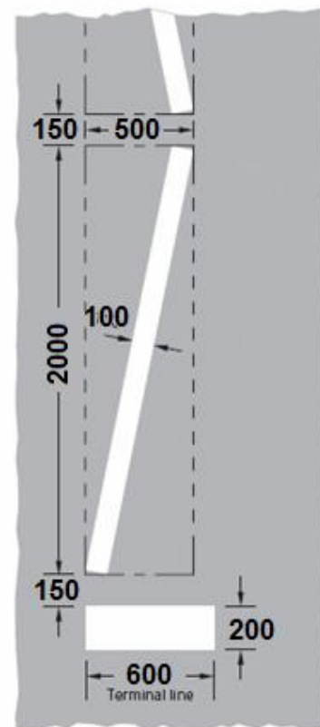
RPC 002: Zigzag and Terminal Line
