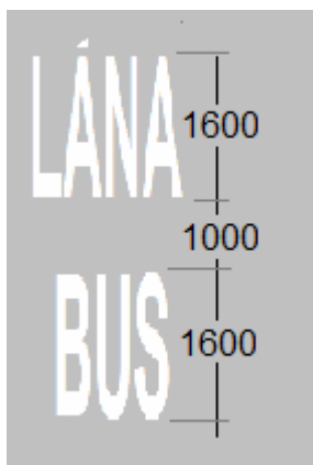
Part of RRM 024: Continuous Bus Lane Line
