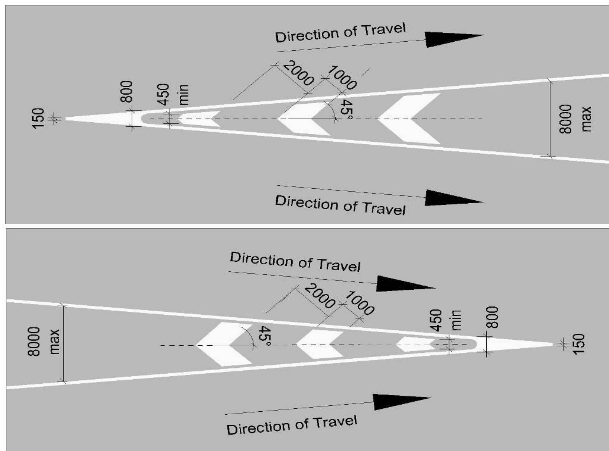
Chevron Markings for Diverging and Merging Traffic on Motorways and Dual Carriageways
