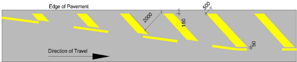
Diagonal Hatched Marking for Use on Nearside of Dual Carriageways
