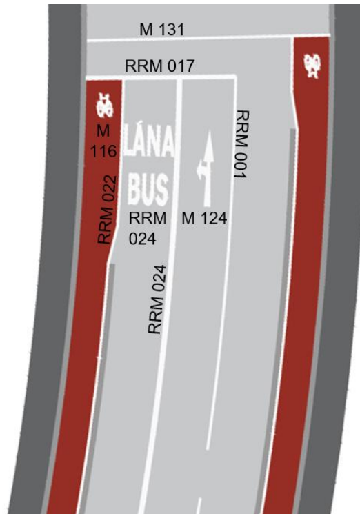
Figure 7.32a: Example road markings for a continuous Bus Lane up to the junction Stop Line
