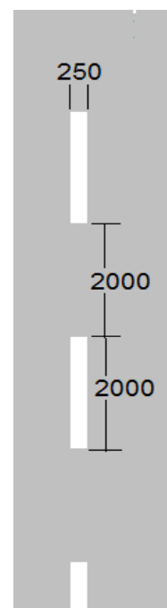
RRM 028: Merge/Diverge Lane Line
