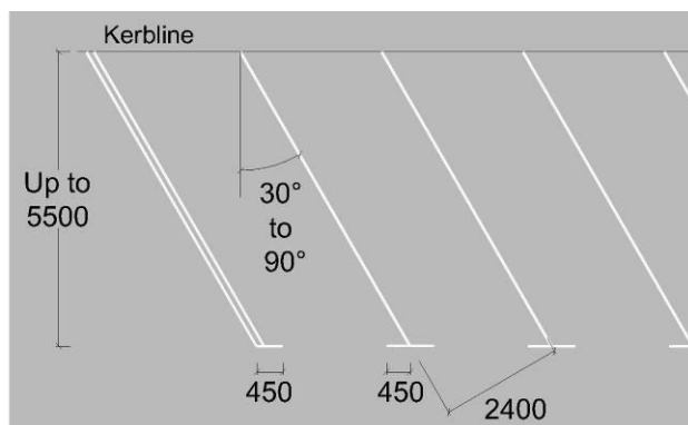
RRM 014: Angled Parking Bay Markings
