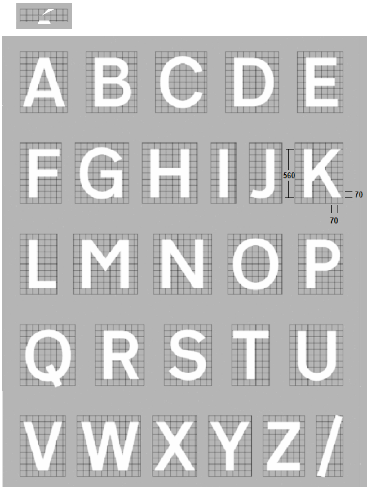
Figure 7.60: Transport Medium Base Font
