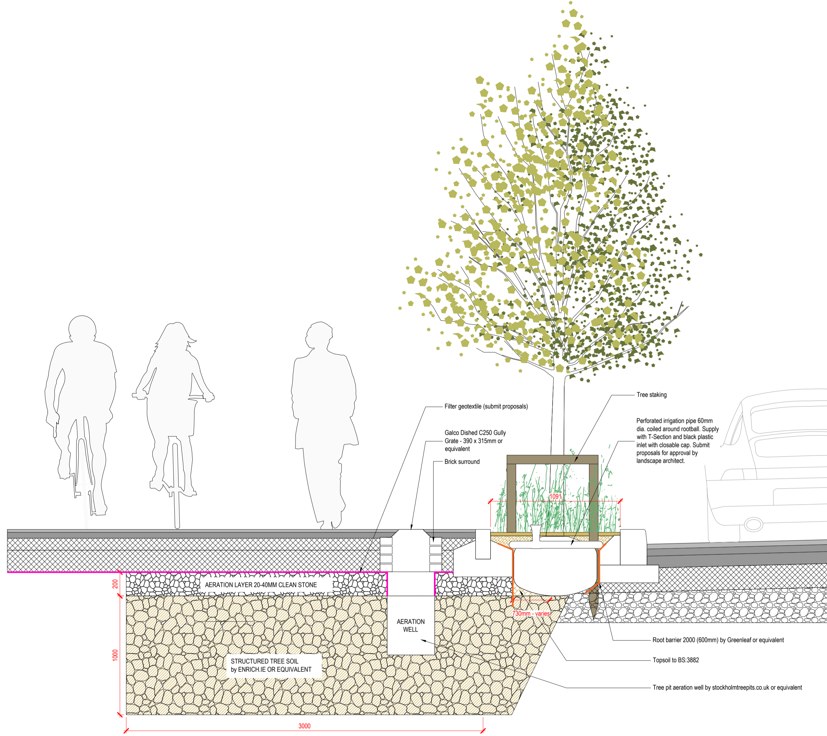
S-01/SECTION 01 - SCALE 1:20
