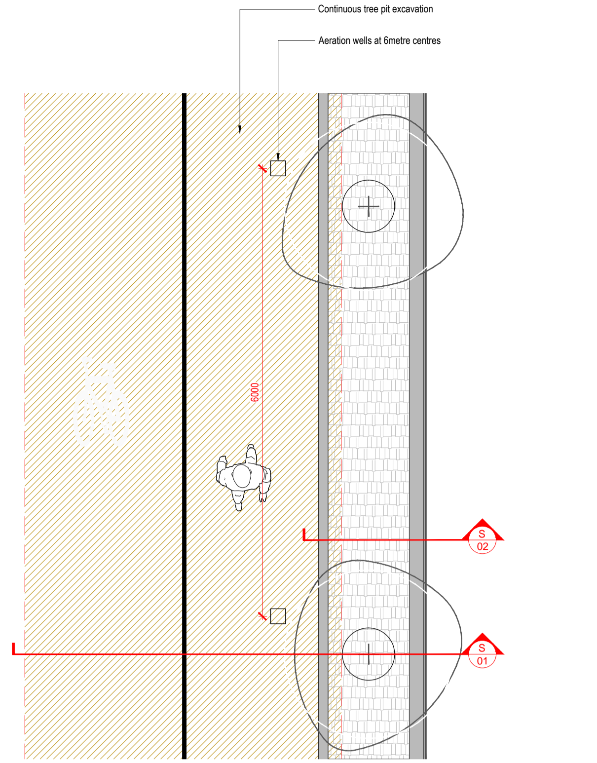
PLAN - SCALE 1:50
