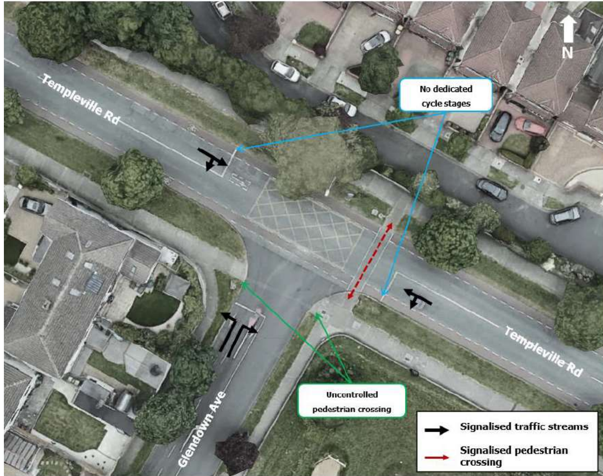
Existing Glendown Road Junction
