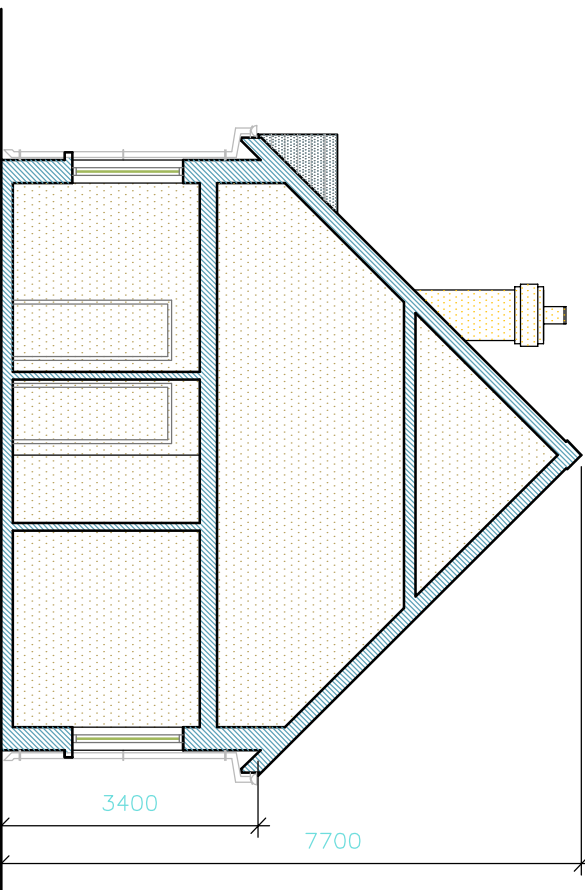
SECTION
