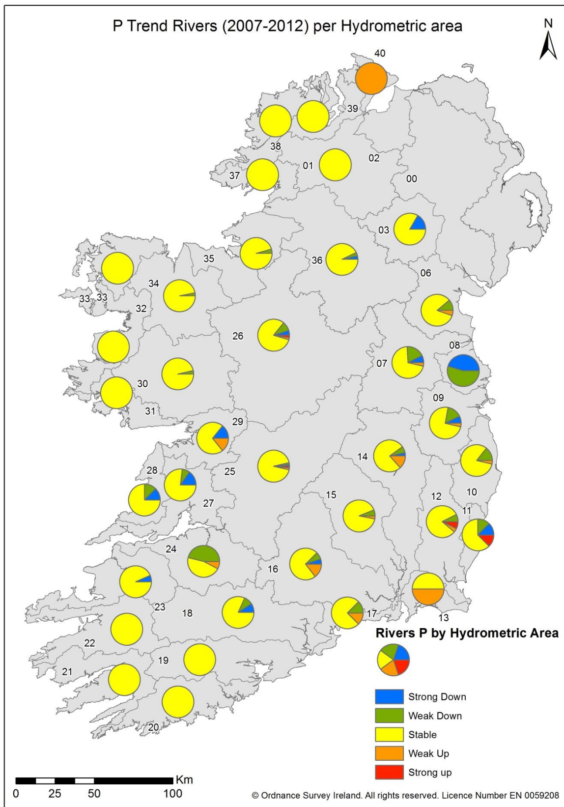
Figure 8: Map showing Orthophosphate trends 2007 – 2012 by Hydrometric area (Source, EPA)
