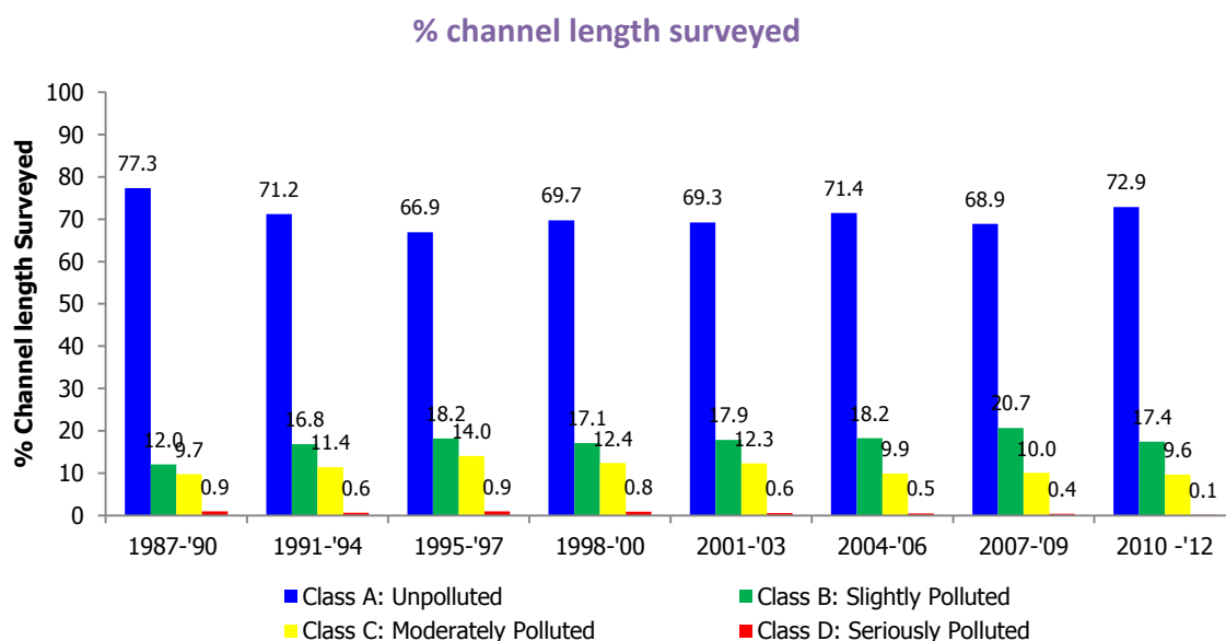
Figure 5: Trends in the 13,300km baseline showing the percentage of surveyed channel nationally in the four EPA biological quality classes
