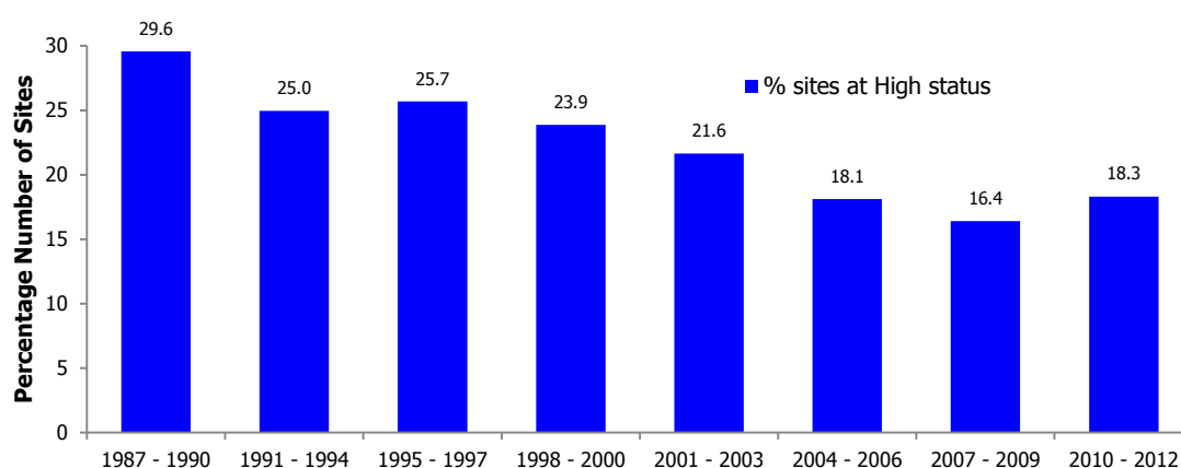
Figure 13: Long-term trends in the percentage number of high ecological quality (Macroinvertebrate) river sites (1987 – 2012).
