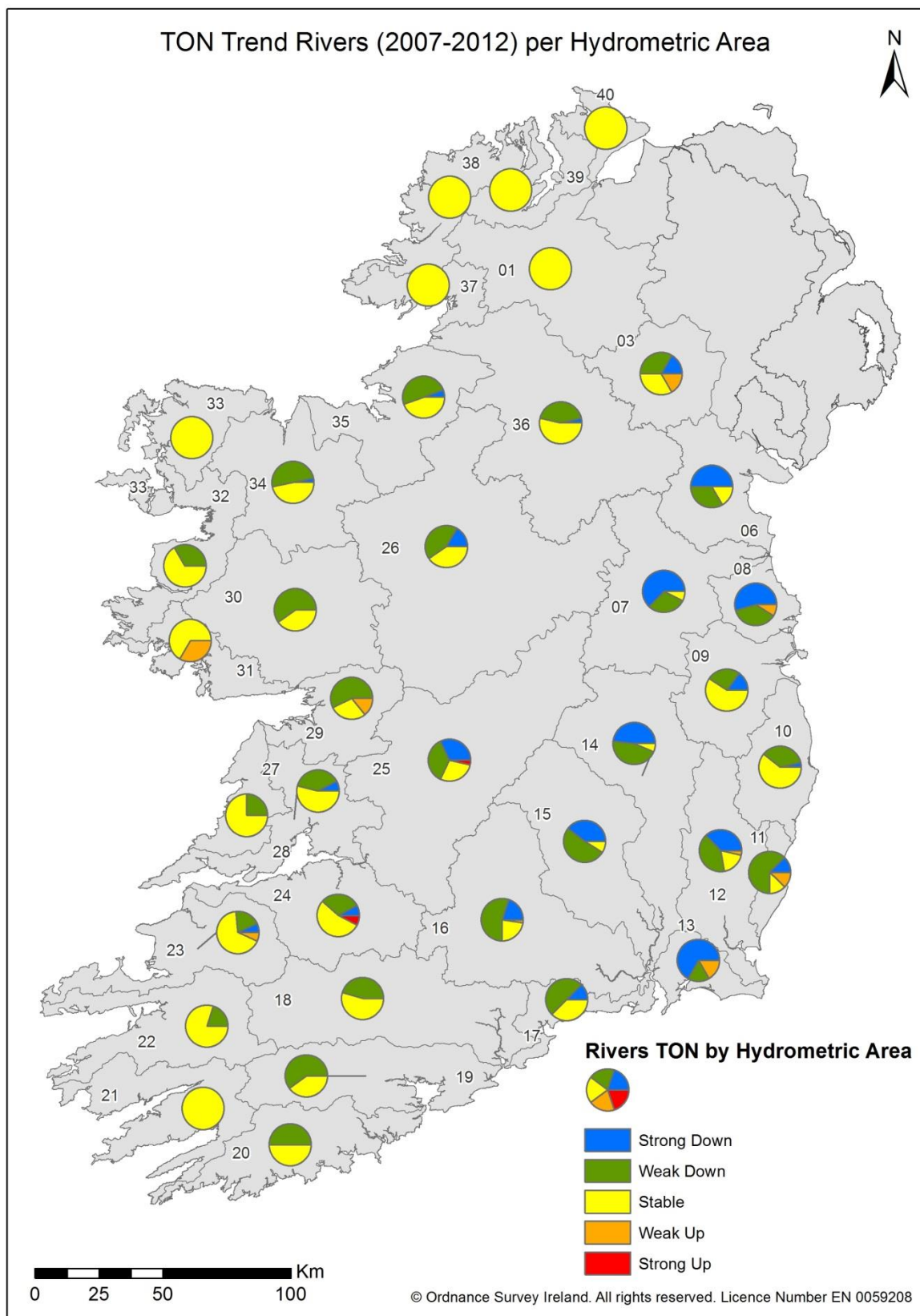
Figure 9: Map showing Total Oxidised Nitrogen (TON) trends 2007 – 2012 by Hydrometric area (Source, EPA)
