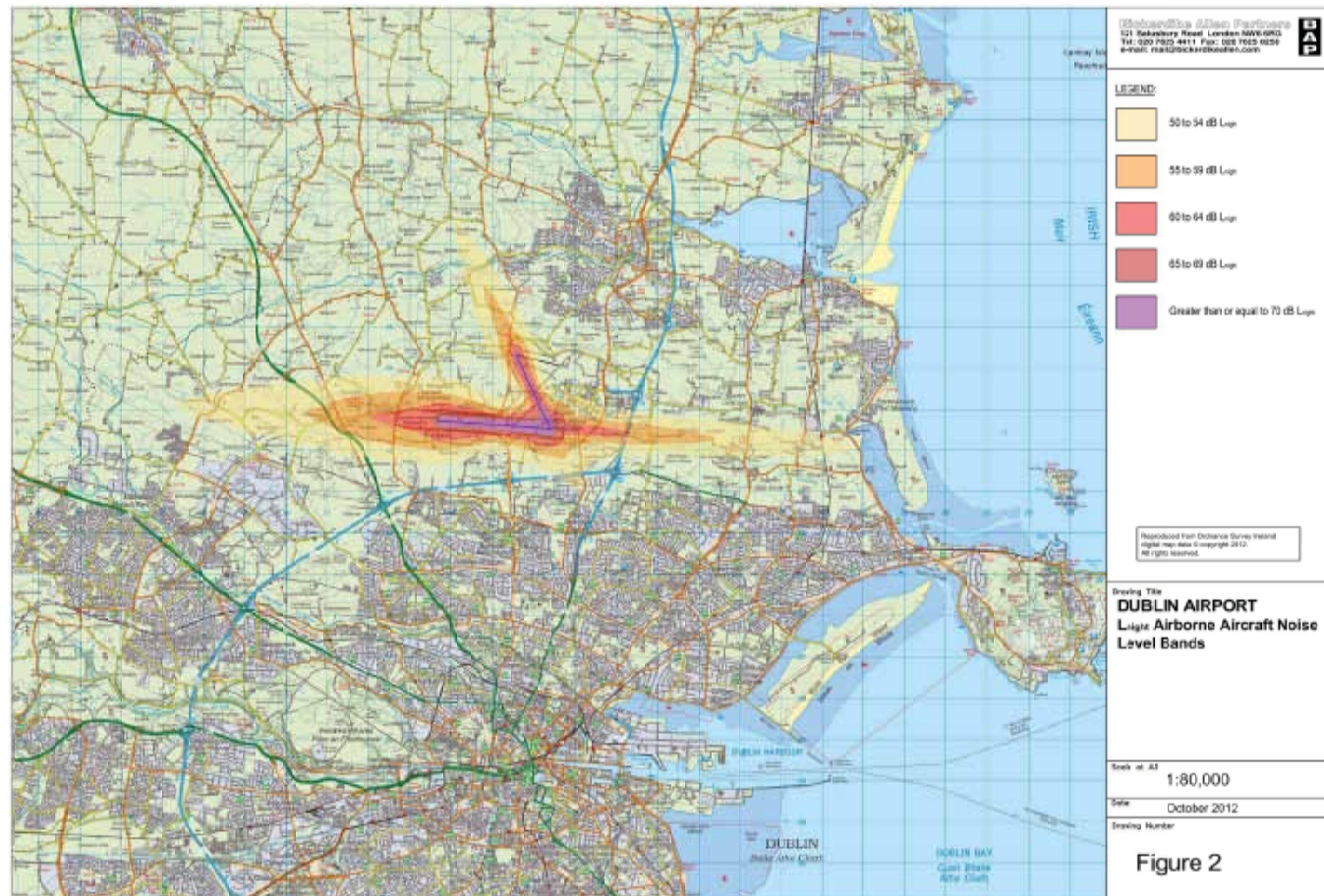
Figure C.4 24-hour Lnight Aircraft Airborne Noise - Dublin Airport
