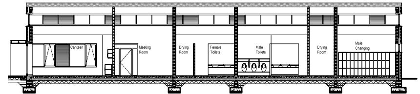
PROPOSED SECTION B-B SCALE 1:100
