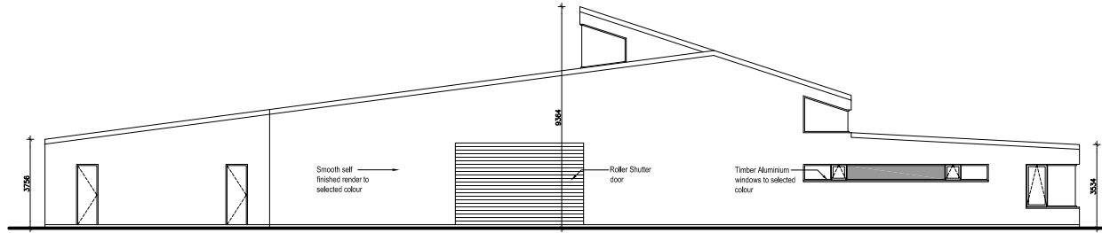
PROPOSED NORTH ELEVATION SCALE 1:100
