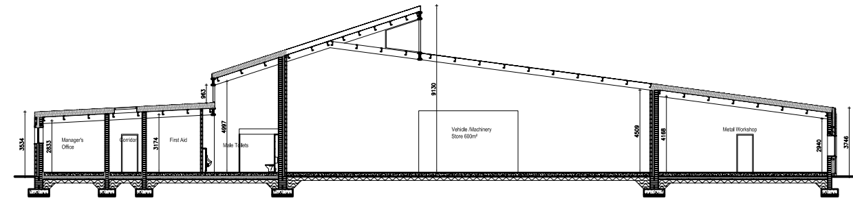
PROPOSED SECTION A-A SCALE 1:100
