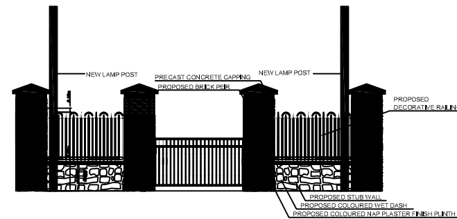
ELEVATION OF PROPOSED PEDESTRIAN ACCESS
