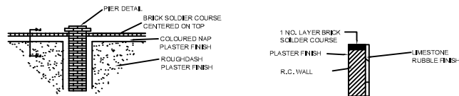
REINFORCED CONCRETE WALL SECTION A-A
