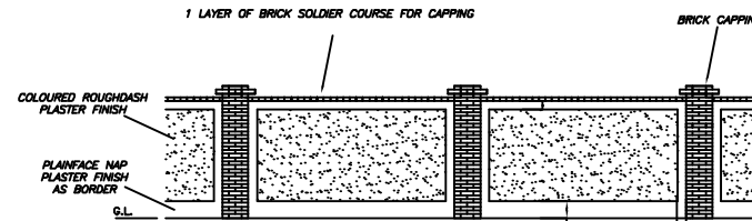
Partial Elevation Of Finished Precast Wall
