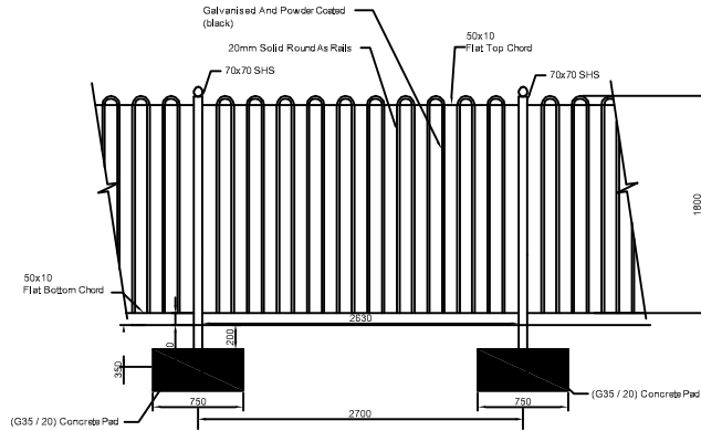
Park Land Fencing Detail Not To Scale
