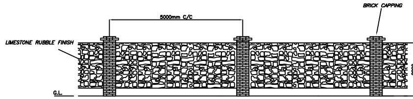
Partial Elevation Of Finished Precast Wall
