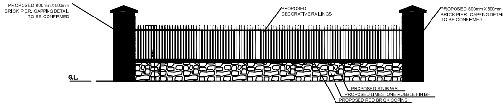
C/WAY ELEVATION OF STUB WALL AND RAILING Scale 1/50
