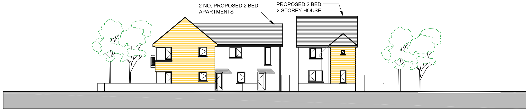
GLENDOHER DRIVE SITE 2 : GLENDOHER DRIVE ELEVATION
